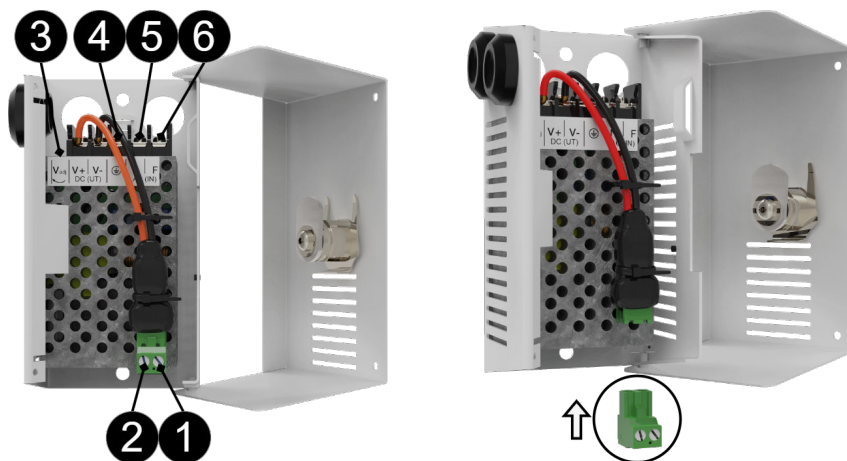
Power Supply 24V 1A and Power Supply 12V 2A.
