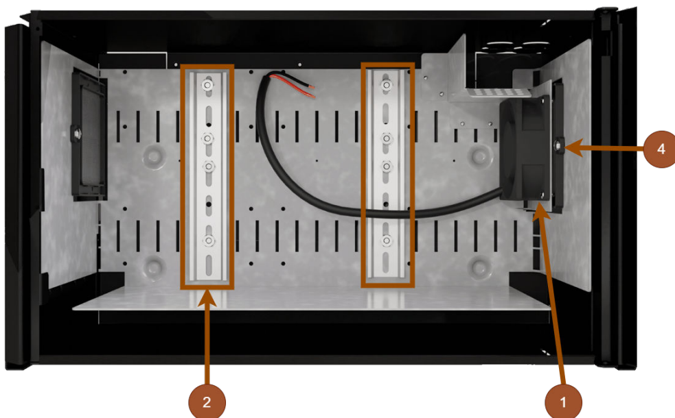
Figure 4. Mount configuration 1
