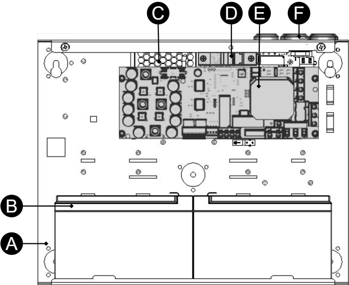
Component overview
