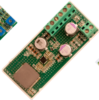
DC converter 24V-12V 6A
